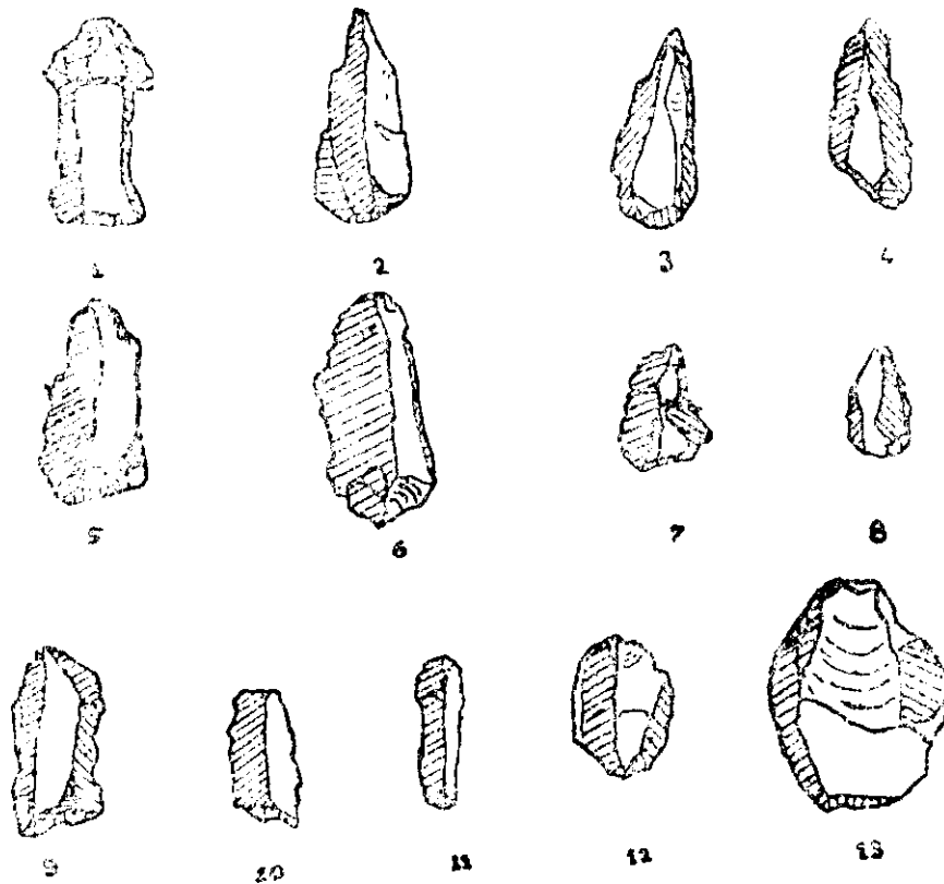
Fig. 2. Microliths from Poona river sand; 5 and 7 carnelian, rest chalcedony; 1 is a unique tanged arrowhead or chisel; the hinged fracture on either shoulder is rare.
