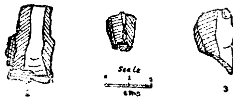
Fig. 3. Quartzite cores (3 carnelian) from which micro-liths have been flaked off.
