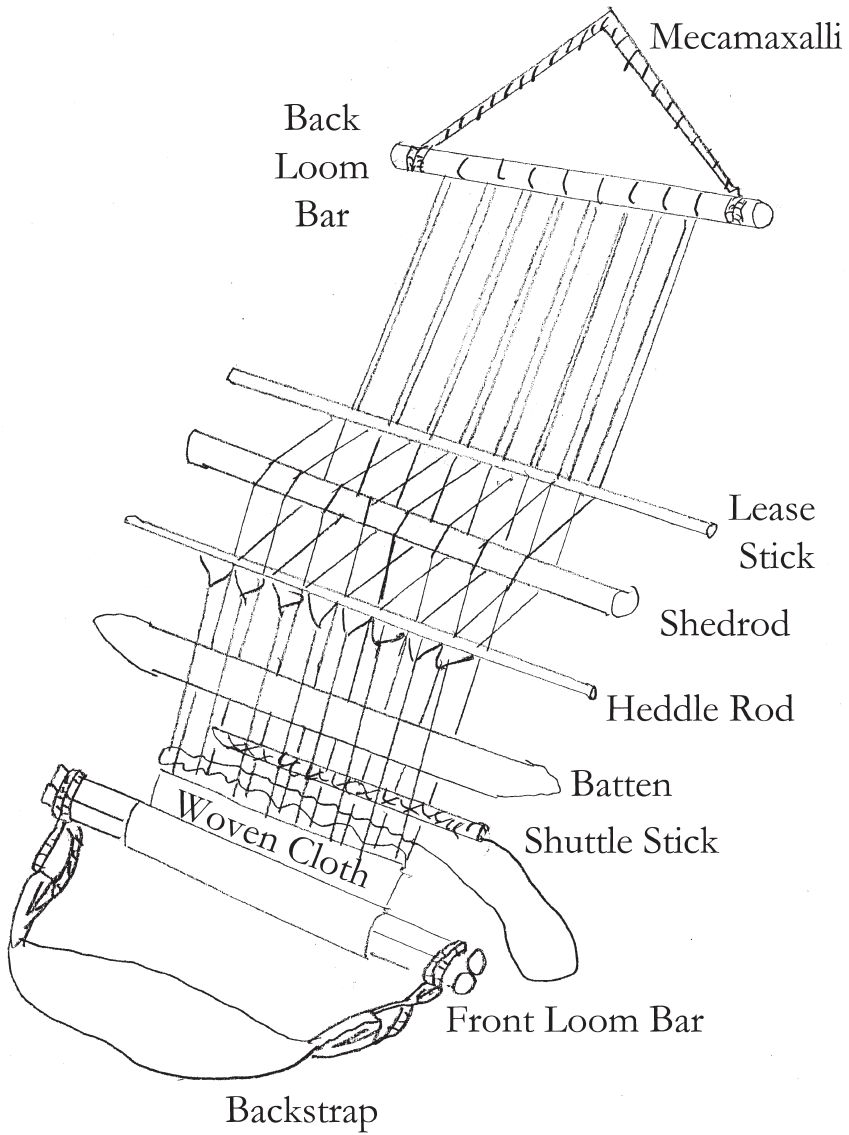
FIGURE 8.4. Backstrap loom and accouterments. (Redrawn from Anderson [1978: 52].)
